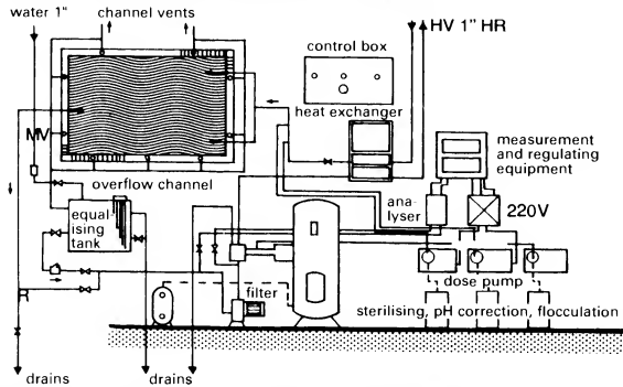
③ Servicing diagram for pool with overflow channel
